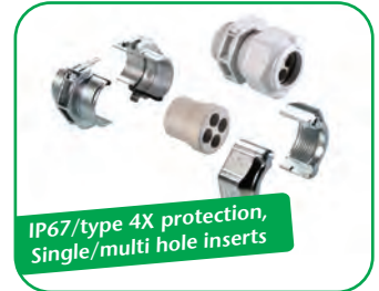
Uni Split Splittable cable gland
